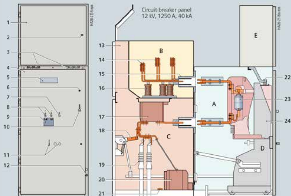
Basic panel design (example)
